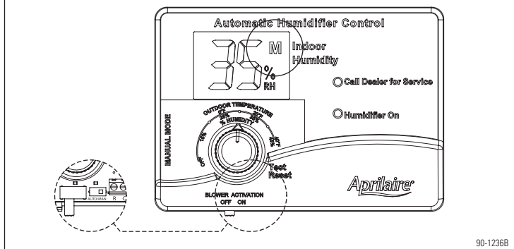
FIGURE 3 – Manual Mode
