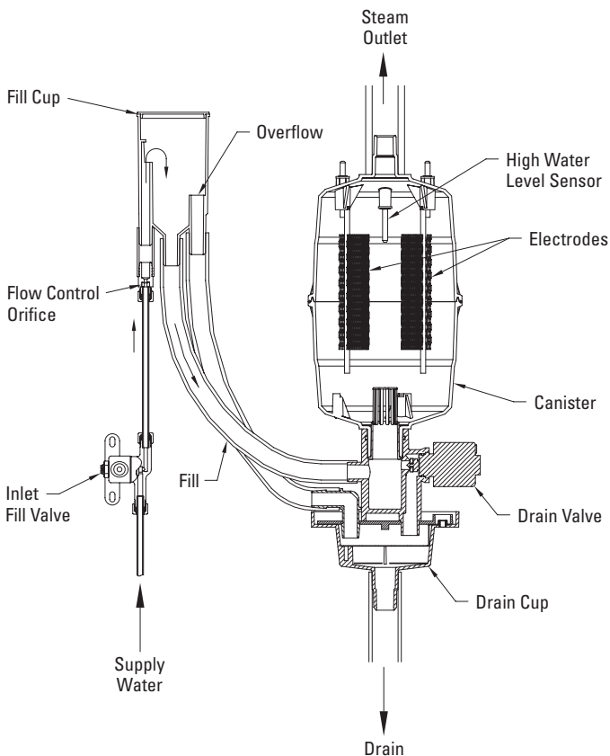
FIGURE 1 – Fill and Drain System and Canister
